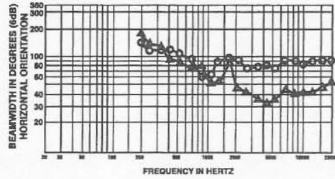
FIGURE 5 — Directivity vs. Frequency
